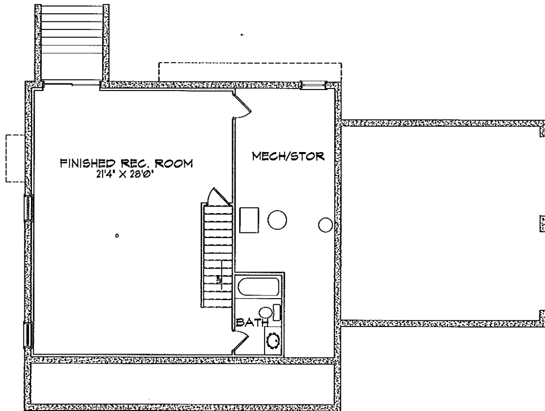
BASEMENT PLAN
