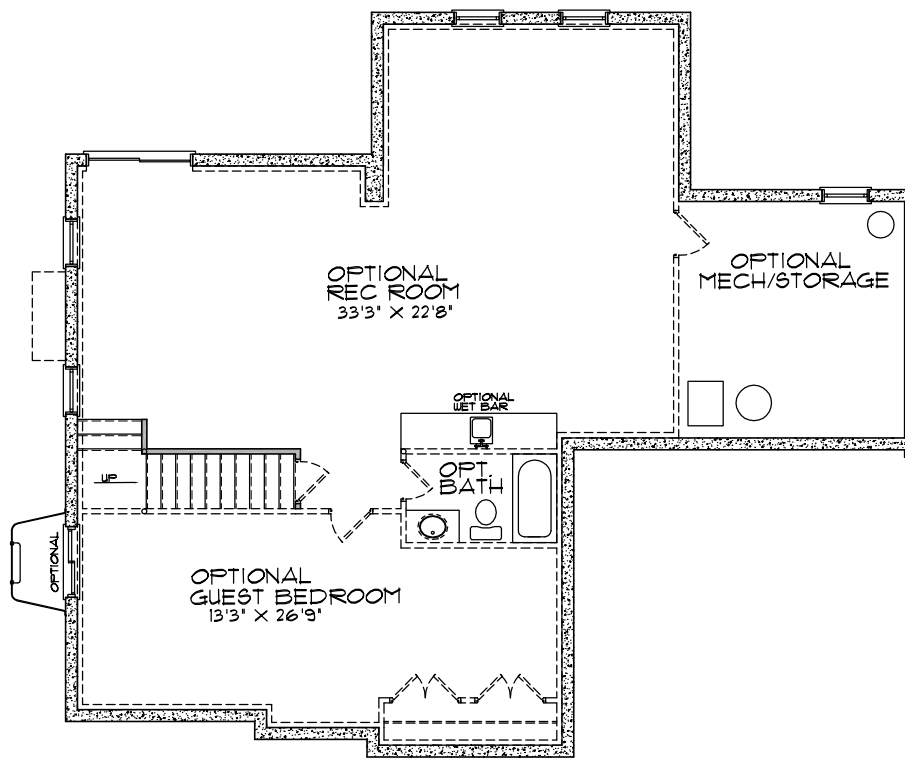
BASEMENT PLAN
